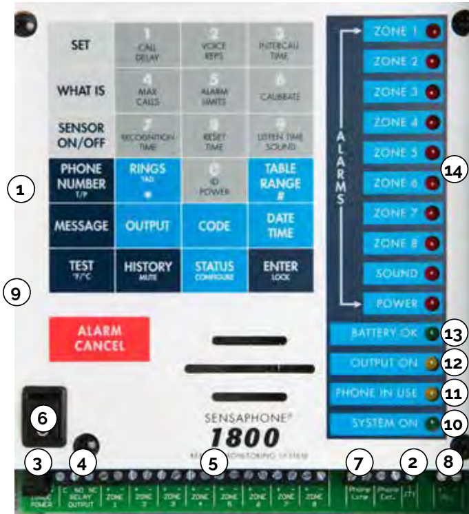
Figure 1: 1800 keypad and terminal blocks
