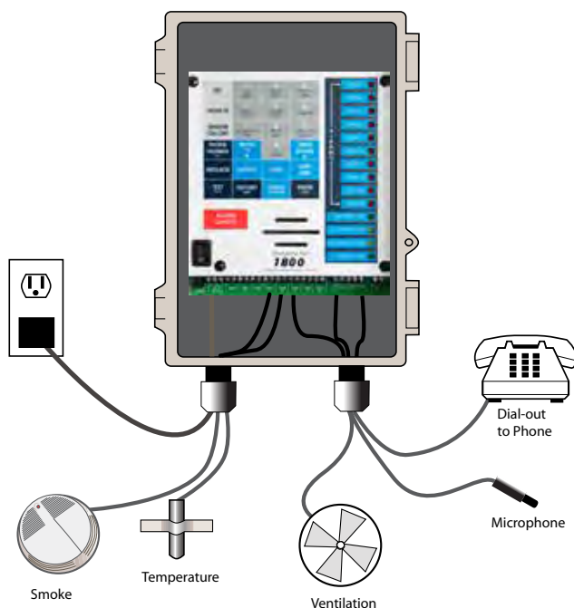
Figure 4: Typical connections from 1800
